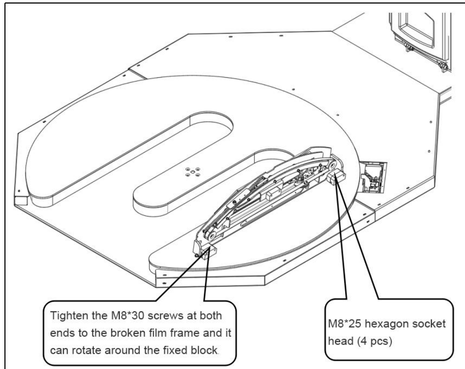
Figure4.5.4.1 Fix film cutting system
