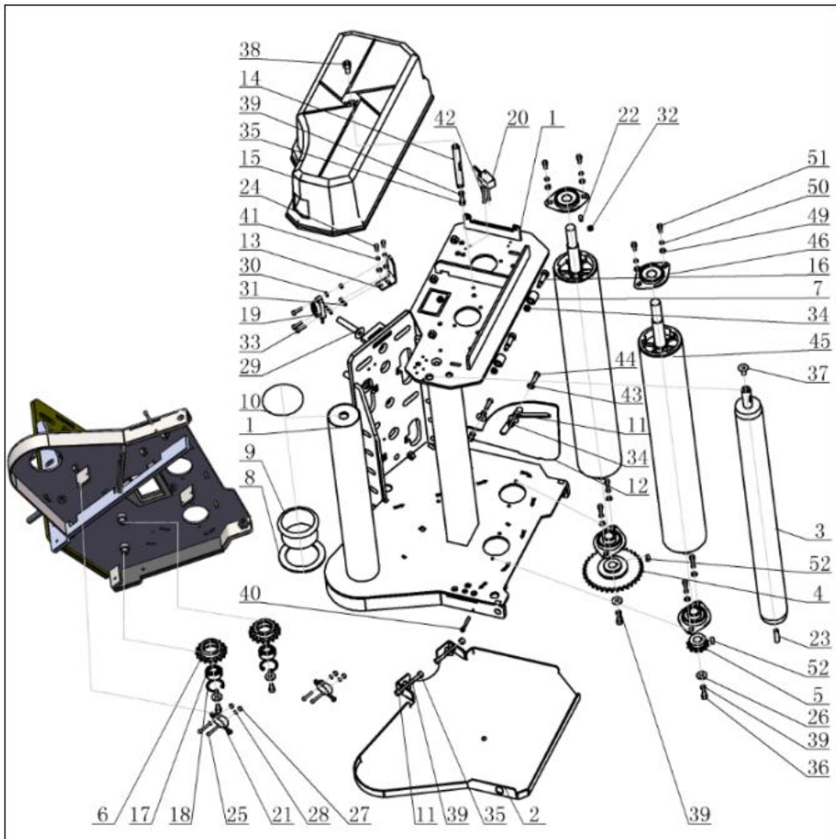
Partially exploded view of film carriage main frame
